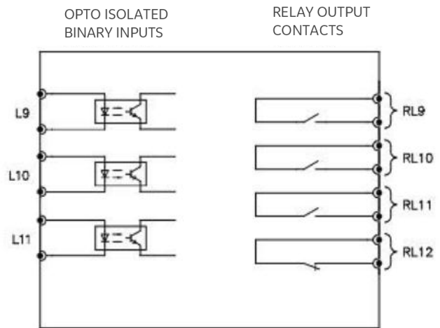
ADDITIONAL 3I + 4O
