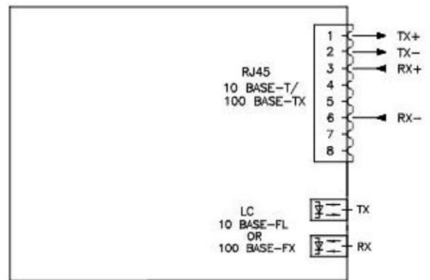
ETHERNET
