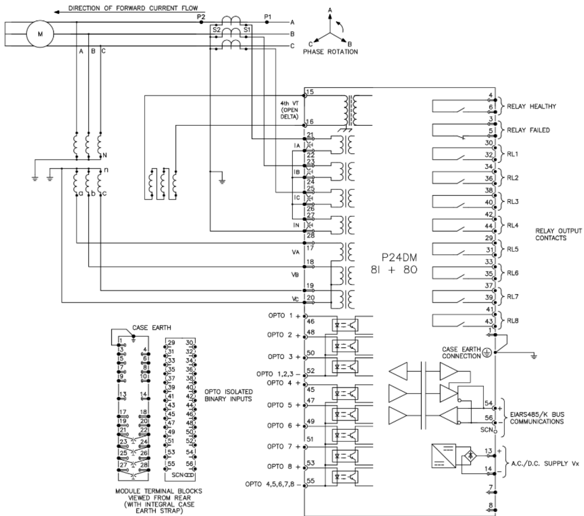
P40 Agile standard hardware (P24DM)
