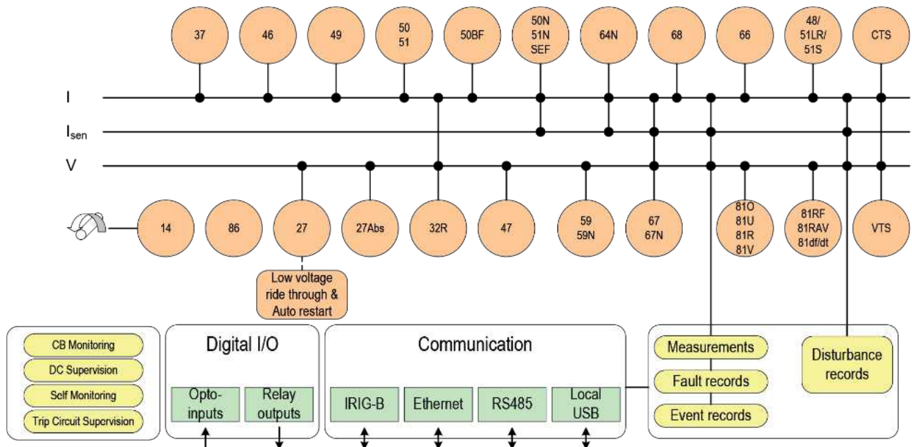
P40 Agile P24xM Functional Diagram
