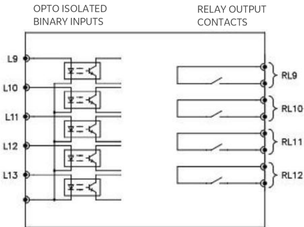
ADDITIONAL 5I + 4O
